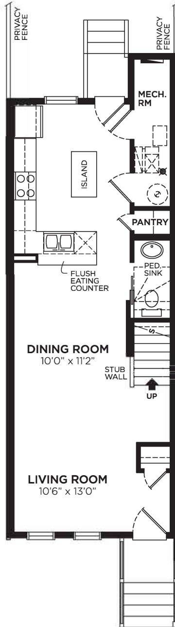
MAIN FLOOR 565 SQ. FT.
